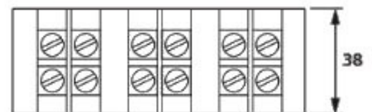
DIN RAIL MOUNTED (2 x clips supplied)
